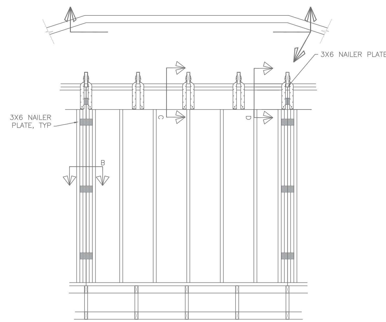
DETAIL A3 WALL PANEL ON CRAWLSPACE/BASEMENT SCALE: 1/2"=1'-0"
