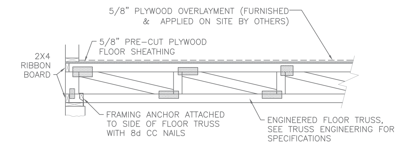
DETAIL C TYPICAL FLOOR TRUSS SCALE: 1/2"=1'-0"
