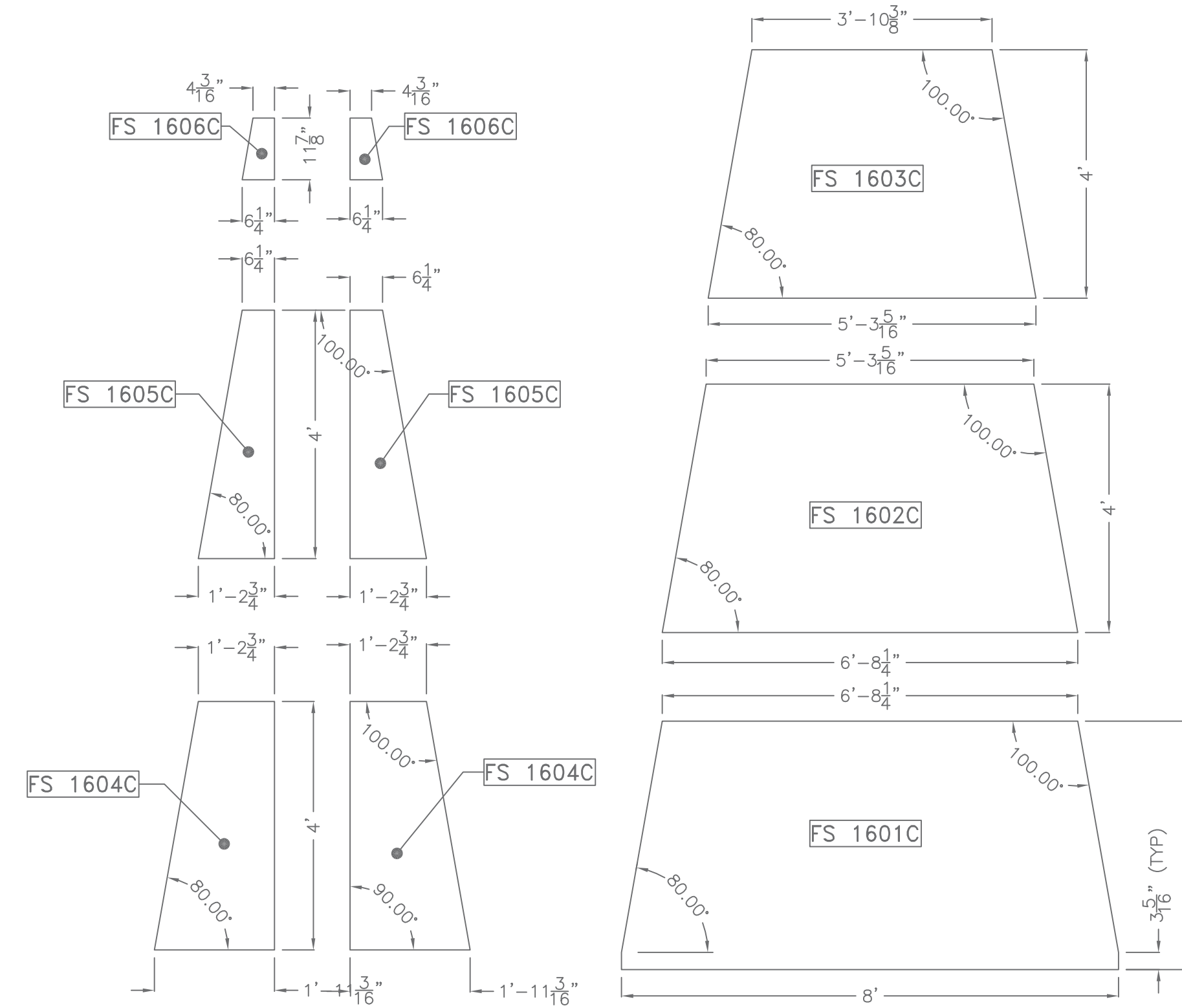
DETAIL B FLOOR SHEATHING COMPONENT DETAILS SHEATHING MATERIAL: (18 PIECES OF EACH REQUIRED) 5/8" CDX PLYWOOD SCALE: 1/2"=1'-0"
