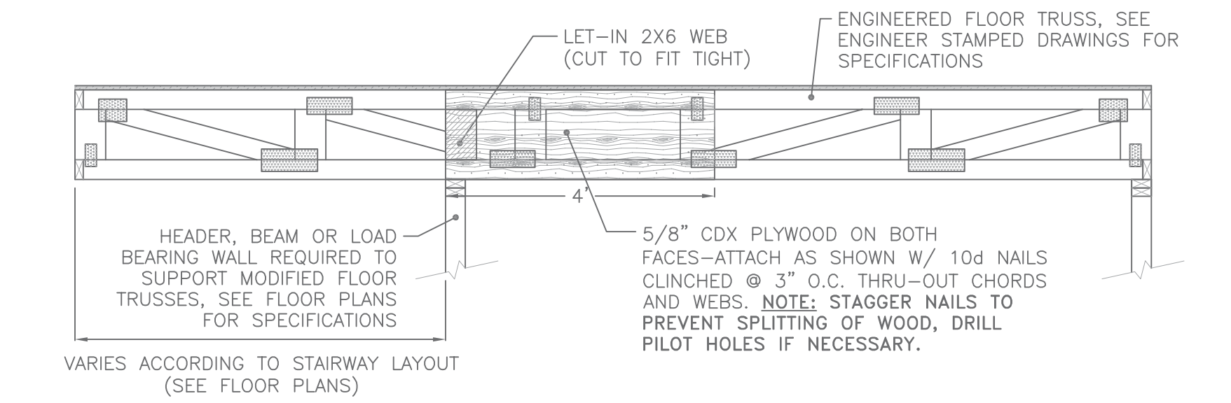
DETAIL E FIELD FIX FLOOR TRUSS SCALE: 1/2"=1'-0"
