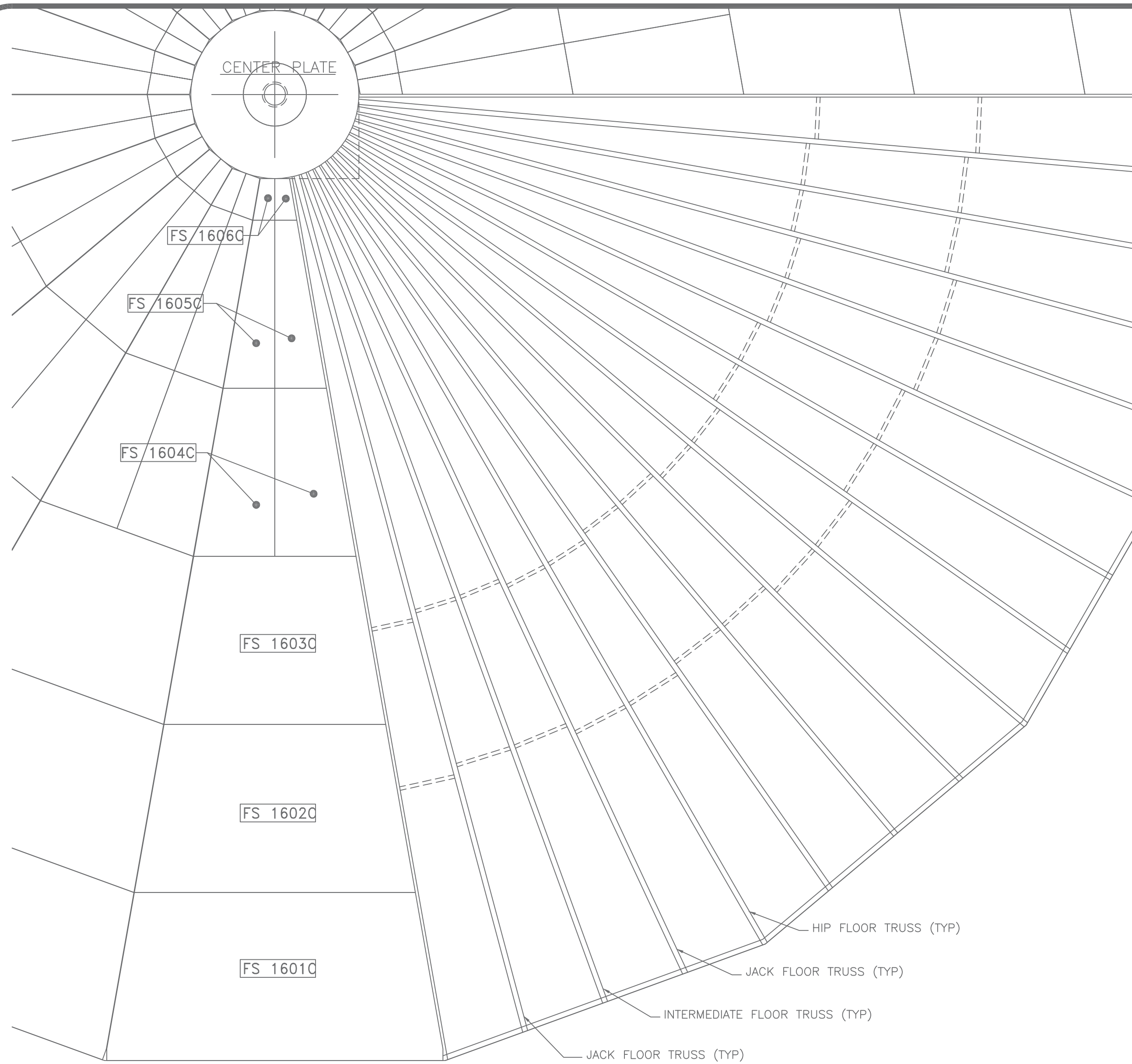
DETAIL A FLOOR SHEATHING PLACEMENT SCALE: 1/2"=1'-0"
