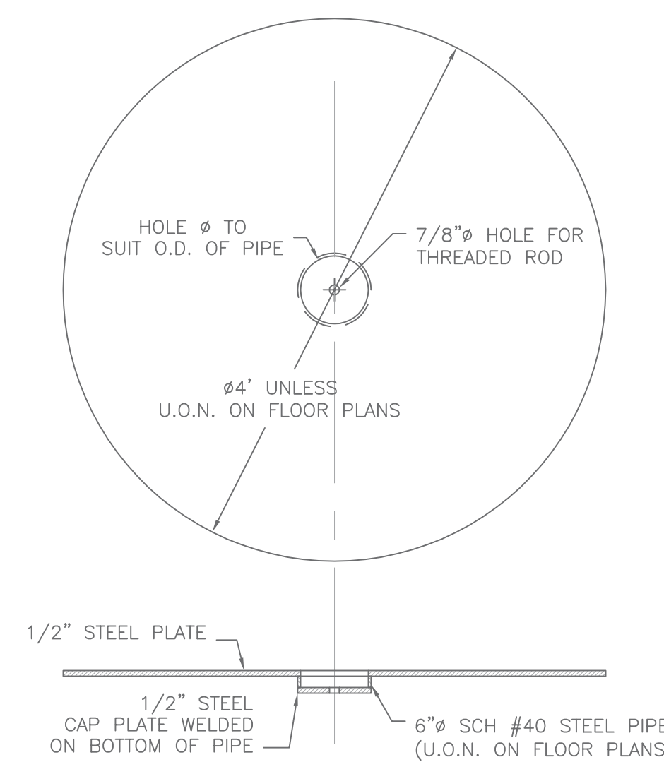
DETAIL F TOP PLATE MODELS 1500-2000 SCALE: 1"=1'-0"
