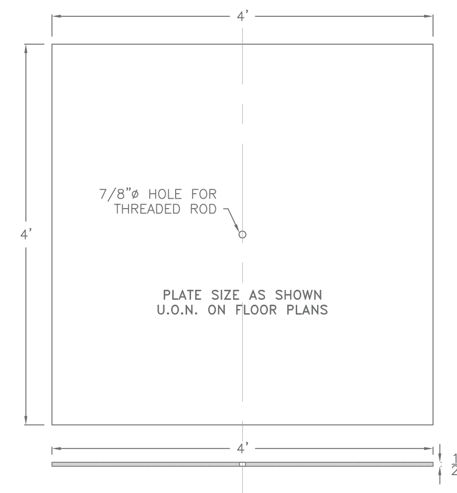
DETAIL G FLOOR PLATE MODELS 1600-2000 SCALE: 1"=1'-0"
