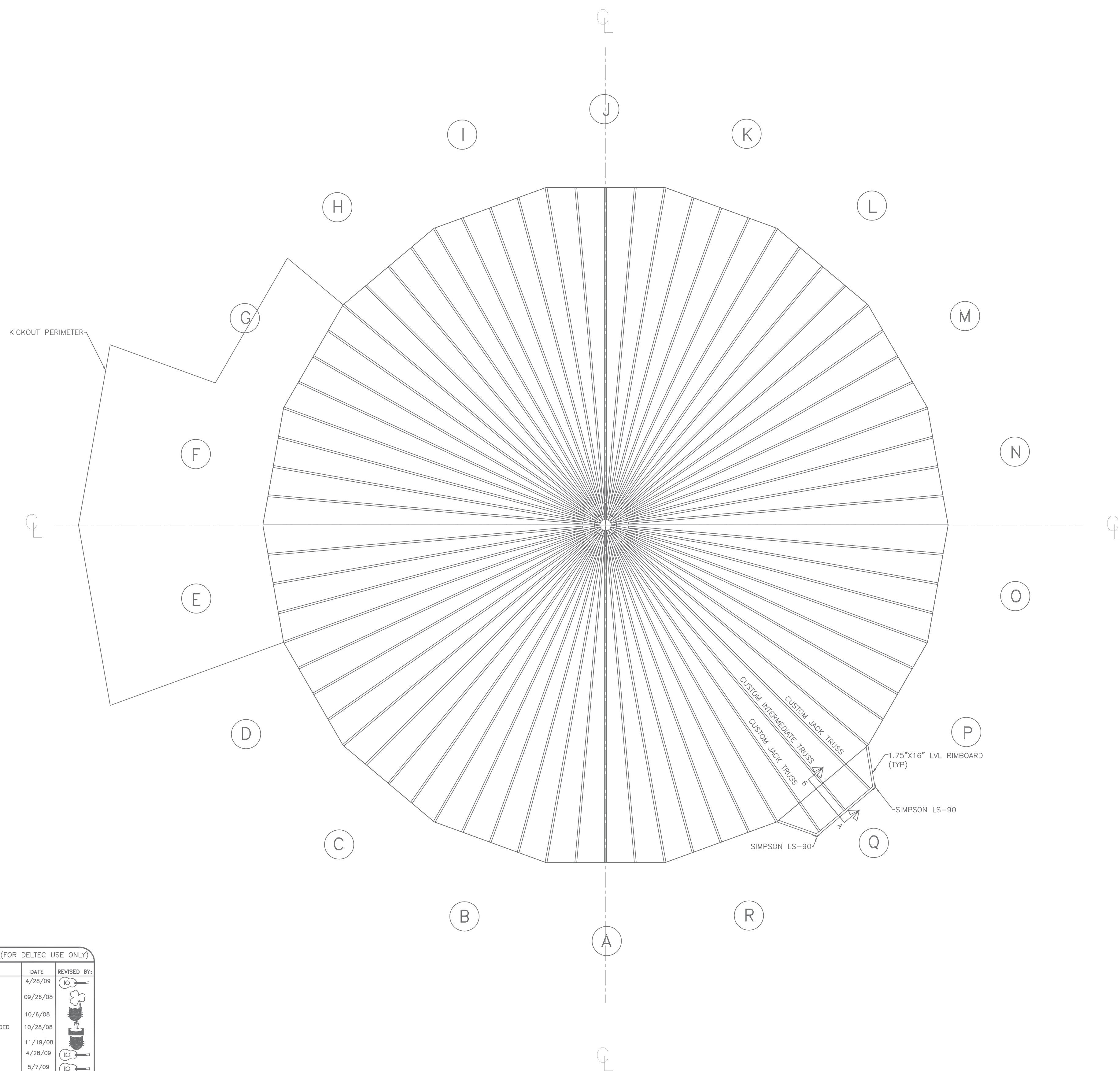
FLOOR TRUSS LAYOUT
